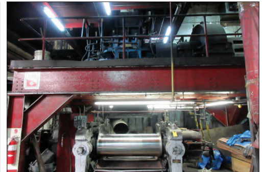
Farrel Bambury Rubber Mixer Mill, Roller Mill, Raw Material
