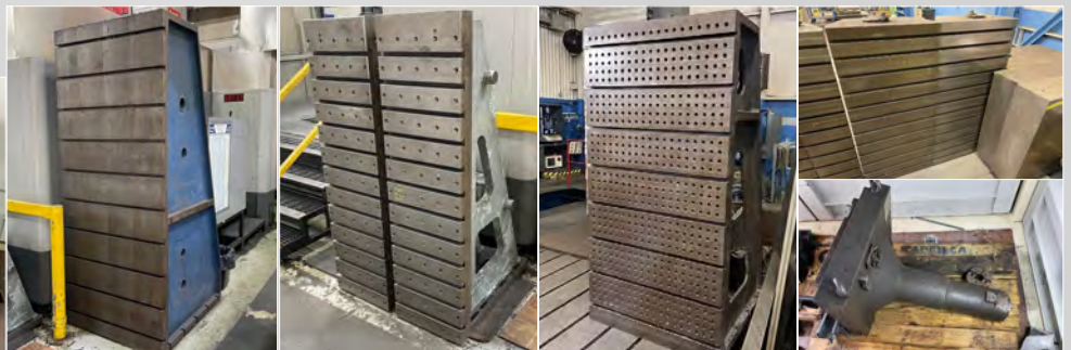
FPT PRAGMA L-60 RAM TYPE TRAVELING COLUMN CNC HORIZONTAL BORING MILL
