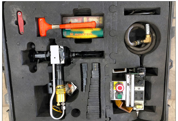
CLIMAX FF3000 Portable Flange Facer
